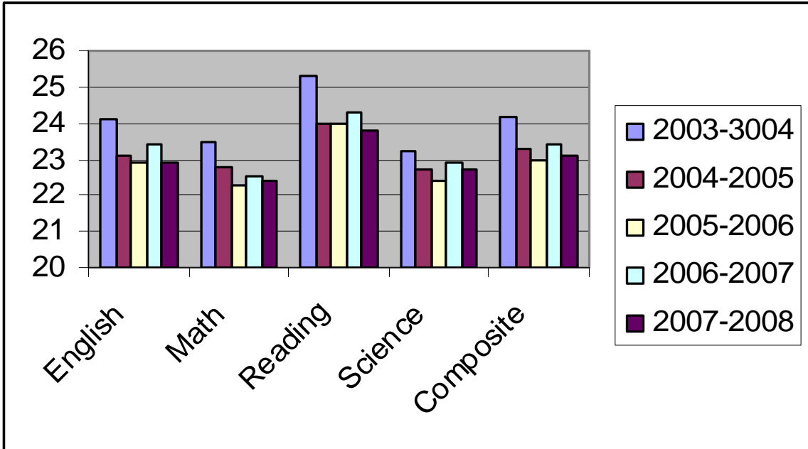
Lawrence Free State ACT Trends 2003-2008
